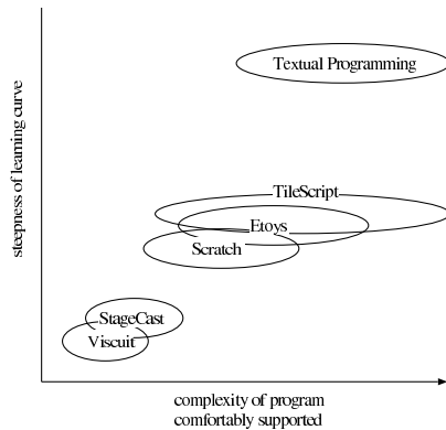
Figure 3. A classification of various end-user programming systems.
